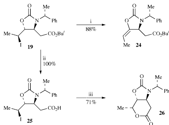
Scheme 8 Reagents and conditions: i, CsOAc, DMF, 20 °C; ii, CF 3 CO 2 H, CH 2 Cl 2 , 20 °C; iii, AgOCOCF 3 , CH 2 Cl 2 , 20 °C.
