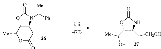
Scheme 9 Reagents and conditions: i, Na, NH 3 (l), EtOH, THF, -78 °C; ii, NH 4 Cl(s), -78 to 20 °C.
