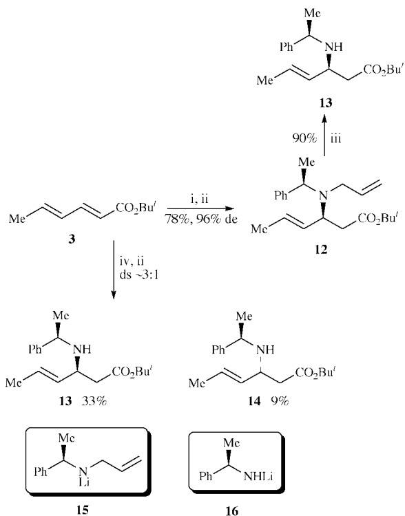
Scheme 4 Reagents and conditions: i, 15 , THF, -78^\circ\text{C} ; ii, \text{NH}_4\text{Cl}(\text{aq}) , -78 to 20^\circ\text{C} ; iii, (\text{Ph}_3\text{P})_3\text{RhCl} , reflux; iv, 16 , THF, -78^\circ\text{C} .
