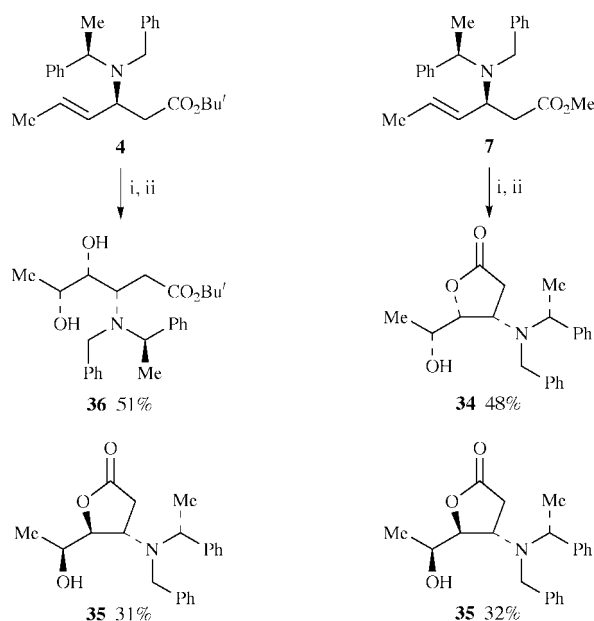
Scheme 11 Reagents and conditions: i, OsO 4 (cat.), K 3 Fe(CN) 6 , K 2 CO 3 , Bu t OH(aq), 20 °C; ii, Na 2 SO 3 (s).
