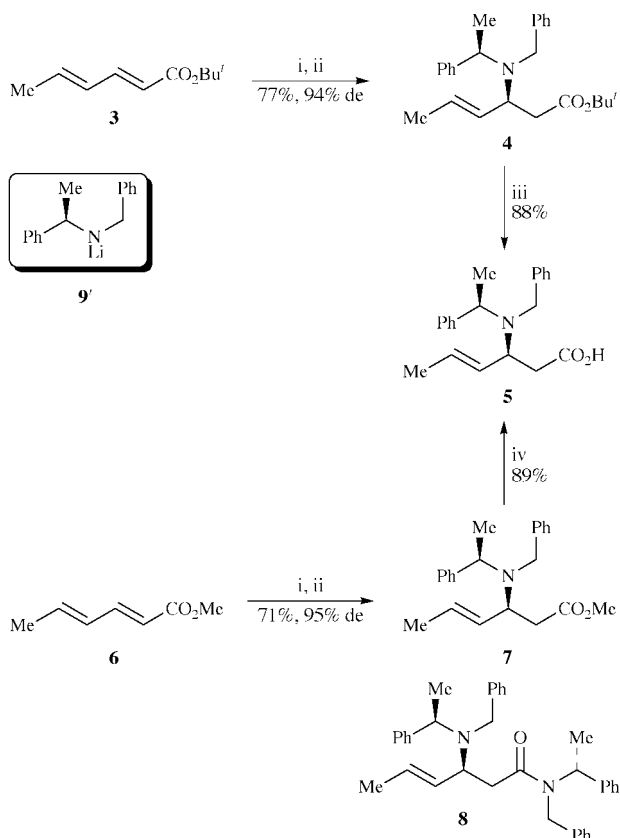
Scheme 2 Reagents and conditions: i, 9' , THF, -78^\circ\text{C} ; ii, \text{NH}_4\text{Cl}(\text{aq}) , -78 to 20^\circ\text{C} ; iii, \text{CF}_3\text{CO}_2\text{H} , \text{CH}_2\text{Cl}_2 , 20^\circ\text{C} ; iv, \text{LiOH} , \text{THF}(\text{aq}) , reflux.
