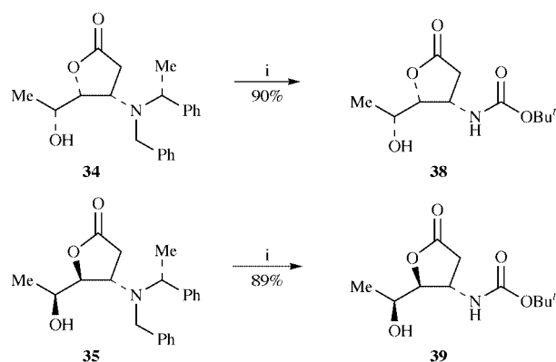
Scheme 13 Reagents and conditions: i, H 2 , Pd(OH) 2 /C, (Bu t OCO) 2 O, EtOAc, 20 °C.
