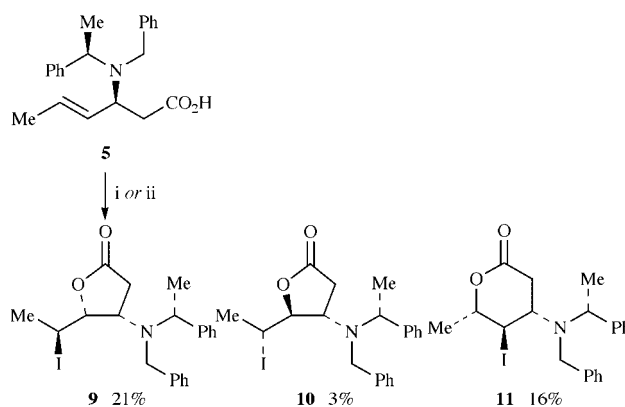
Scheme 3 Reagents and conditions: i, NIS, \text{THF}(\text{aq}) , 20^\circ\text{C} ; ii, \text{I}_2 , \text{Et}_2\text{O} , \text{NaHCO}_3(\text{aq}) , 20^\circ\text{C} .
