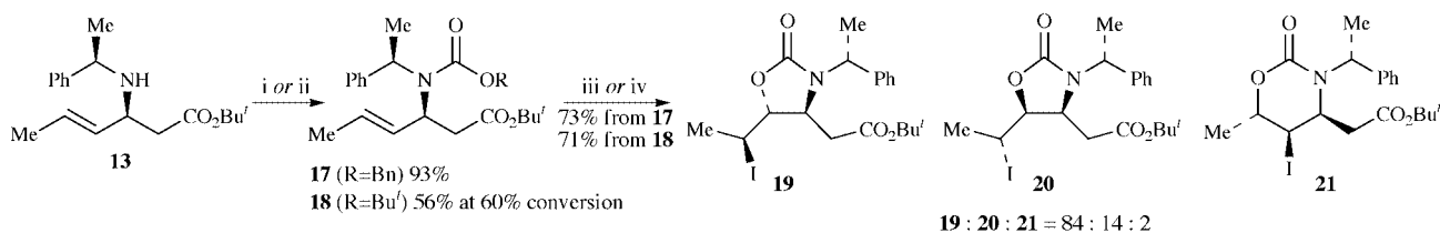
Scheme 5 Reagents and conditions: i, (R = Bn) (\text{BnOCO})_2\text{O} , neat, 20^\circ\text{C} ; ii, (R = Bu t ) (\text{Bu}^t\text{OCO})_2\text{O} , neat, 20^\circ\text{C} ; iii, (R = Bn) \text{I}_2 , \text{CH}_2\text{Cl}_2 , 20^\circ\text{C} ; iv, (R = Bu t ) NIS, THF(aq), 20^\circ\text{C} ; or \text{I}_2 , \text{Et}_2\text{O} , \text{NaHCO}_3(\text{aq}) , 20^\circ\text{C} .
