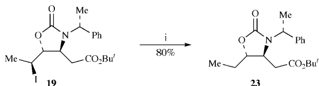
Scheme 7 Reagents and conditions: i, Bu 3 SnH, AIBN, PhMe, reflux.
